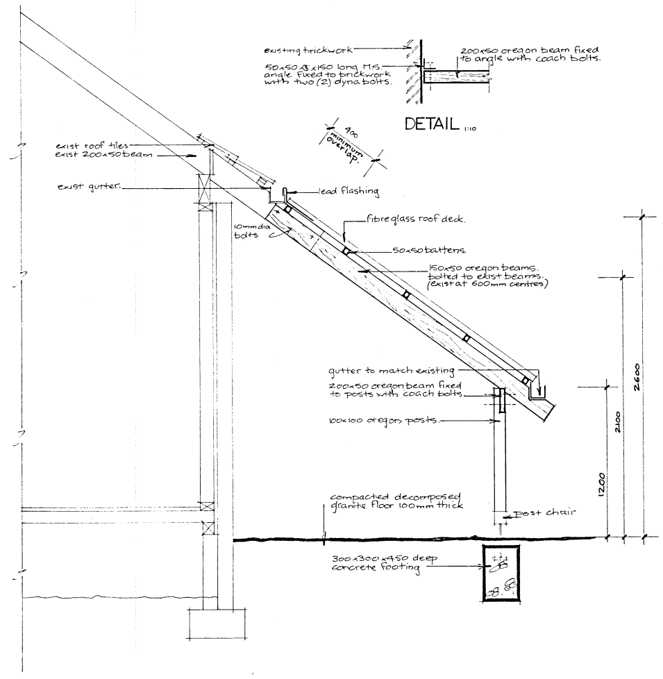
SECTION 1:20
