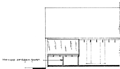
FRONT 1:100
